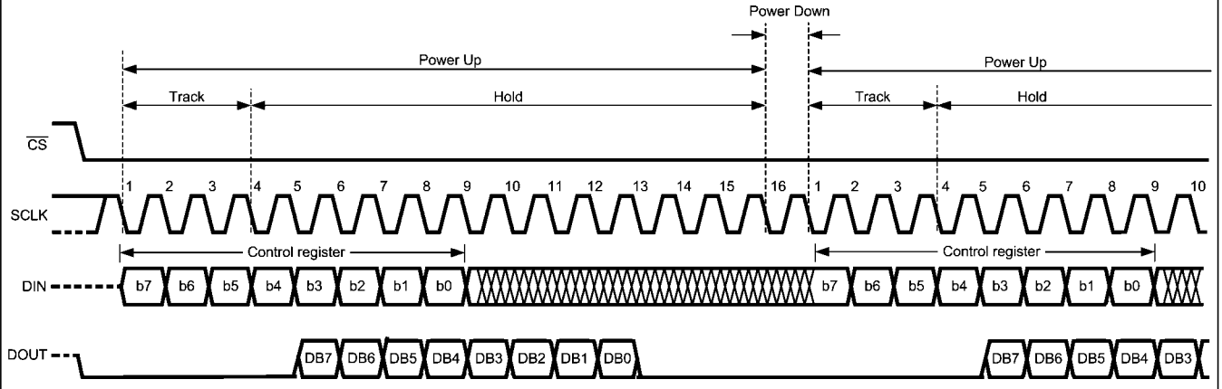
ADC084S101 Operational Timing Diagram
